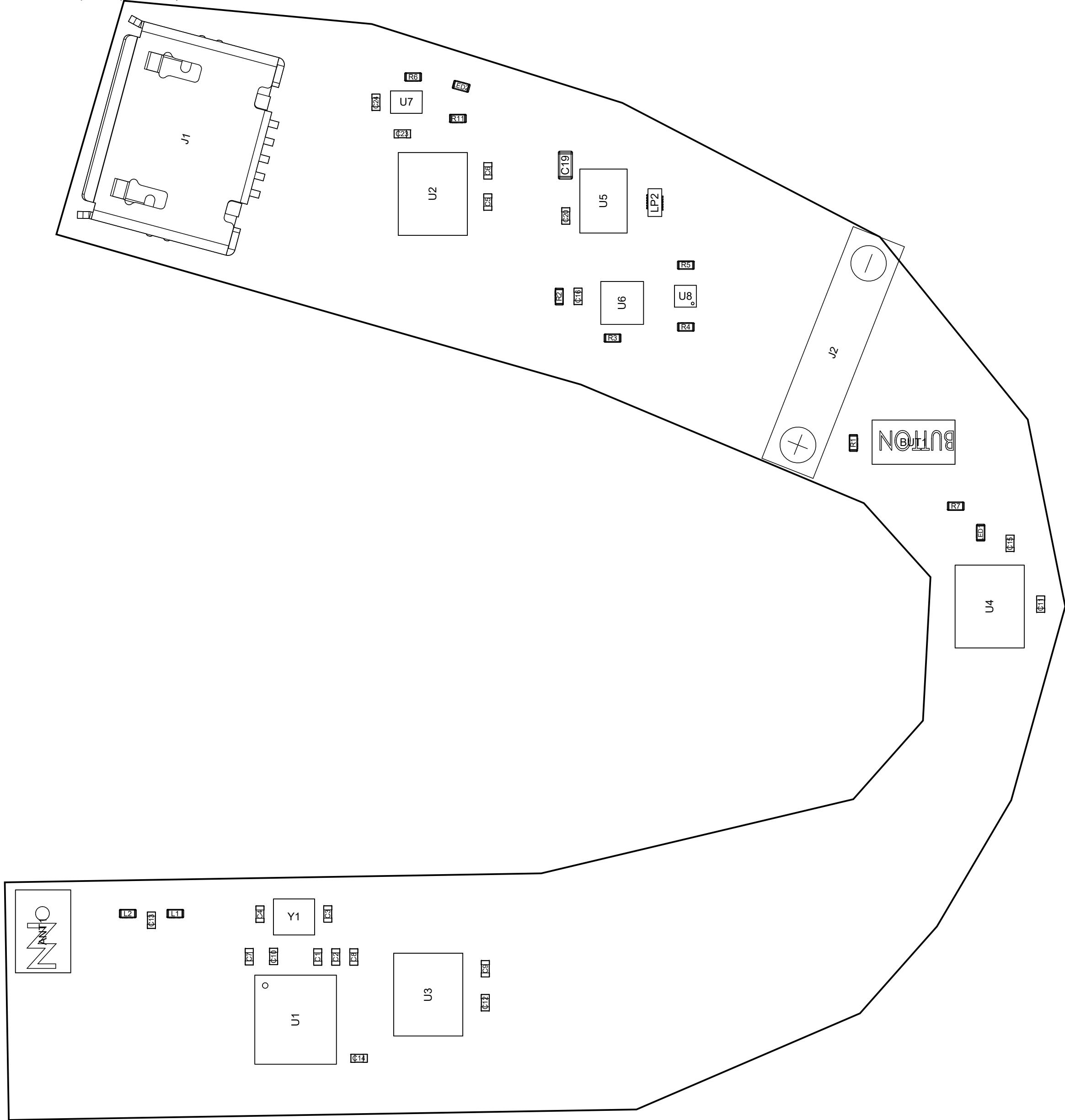
View from Top side (Scale 8:1)
