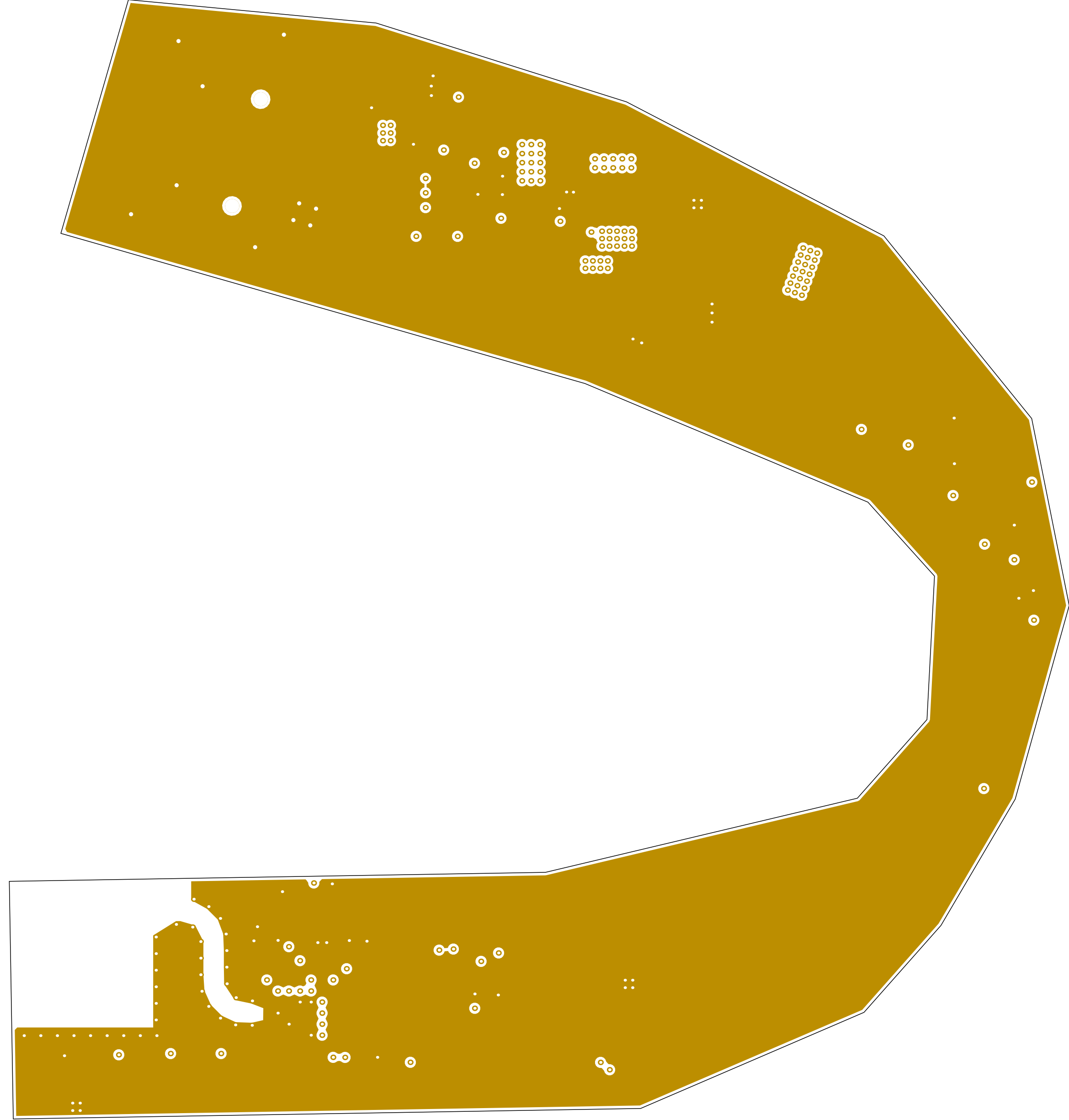
GND (Scale 8:1)
