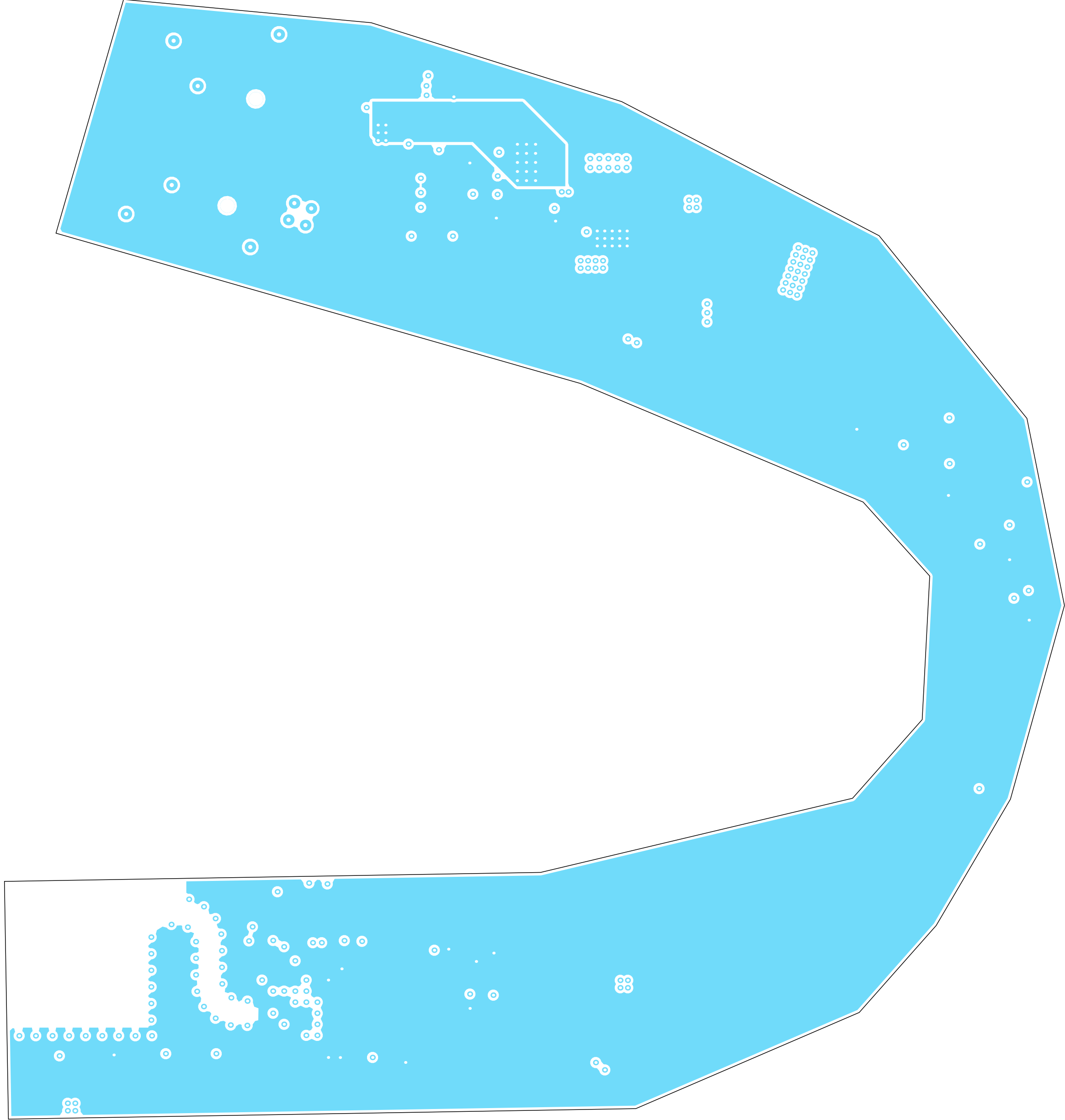
POWER (Scale 8:1)
