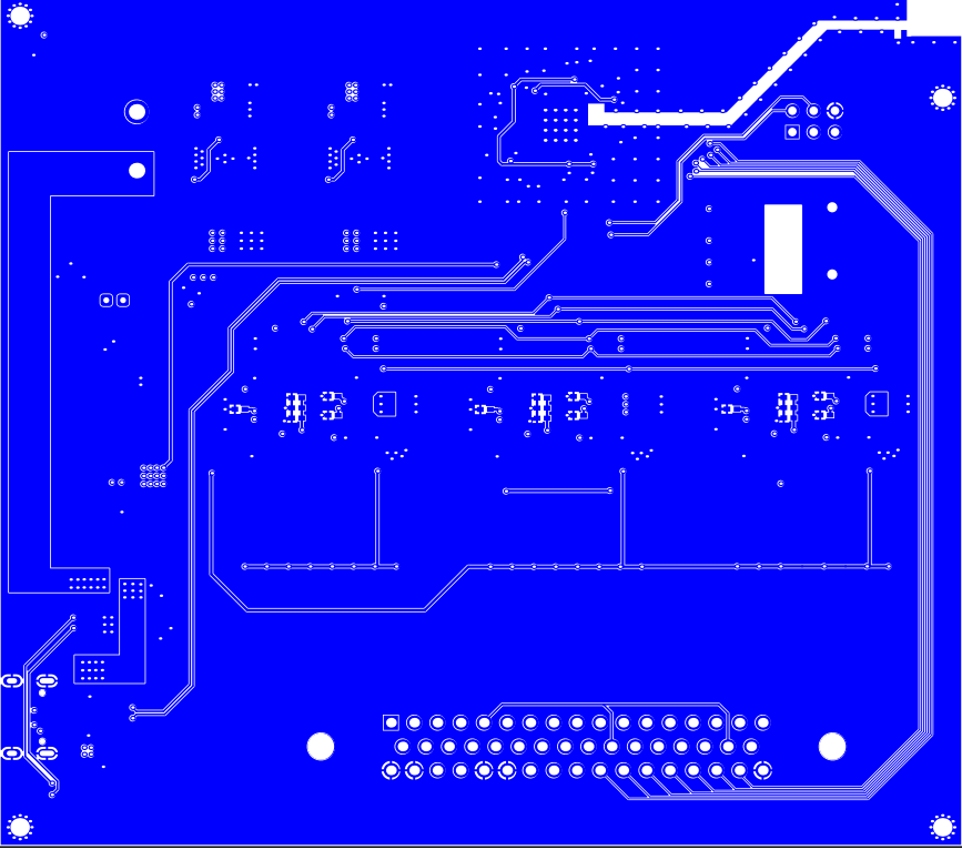
L4 - SIGNAL (Scale 1:1)
