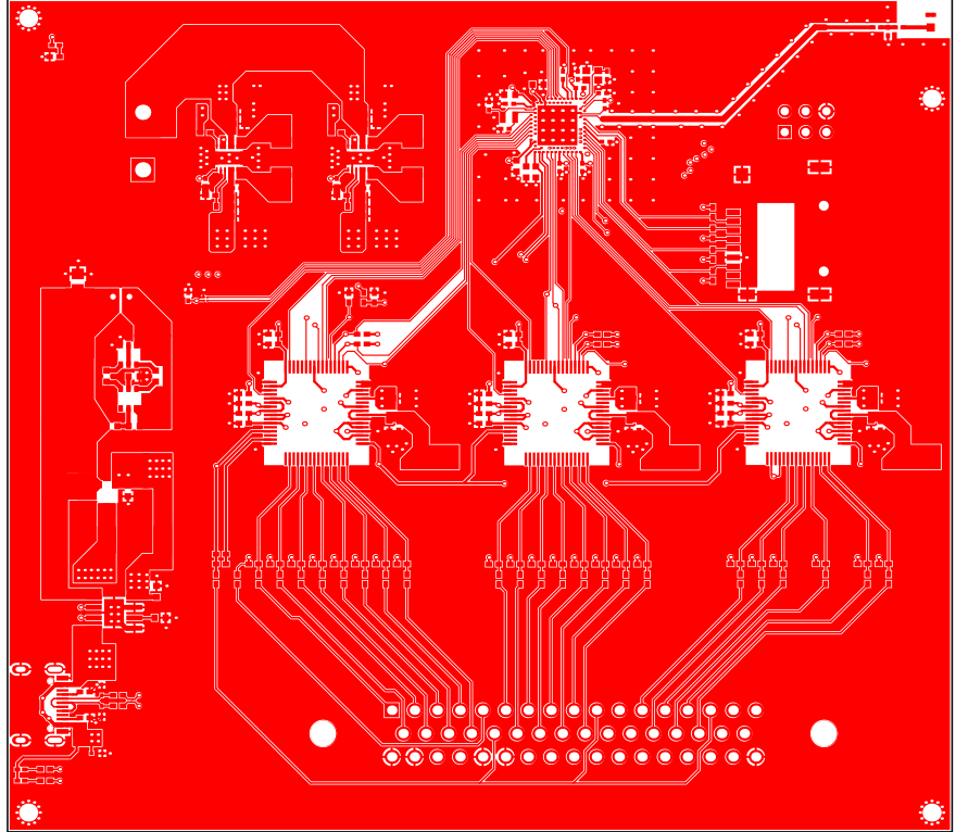
L1 - Signal (Scale 1:1)
