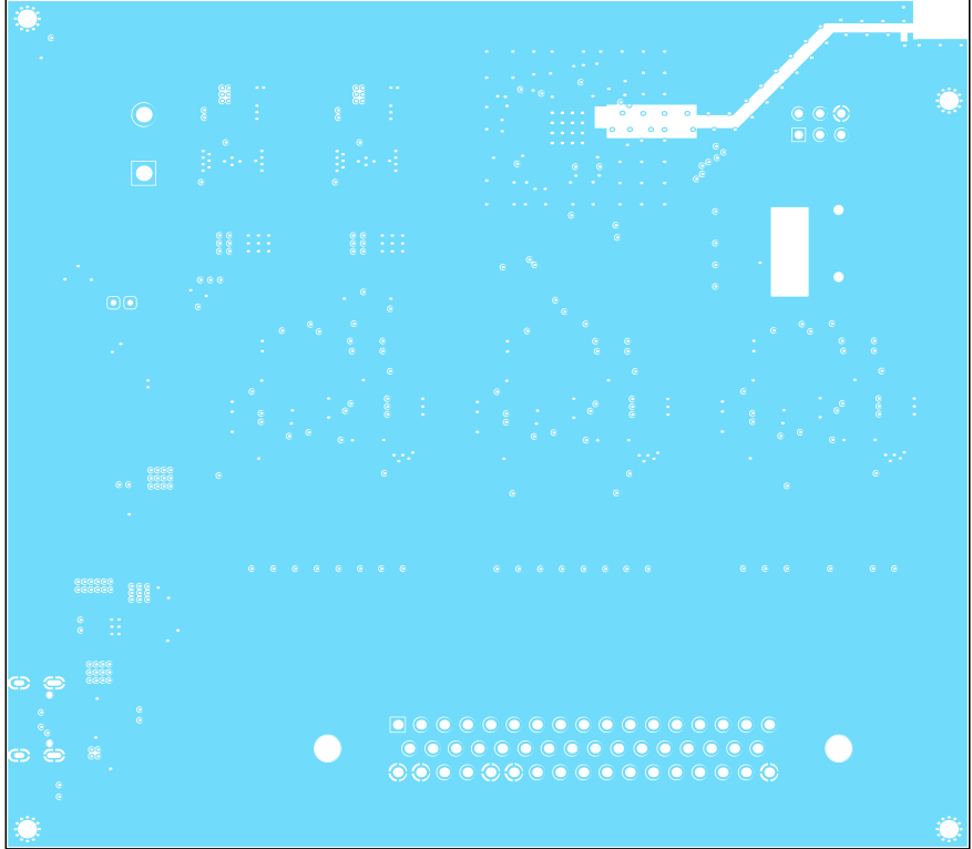
L3 - GROUND (Scale 1:1)
