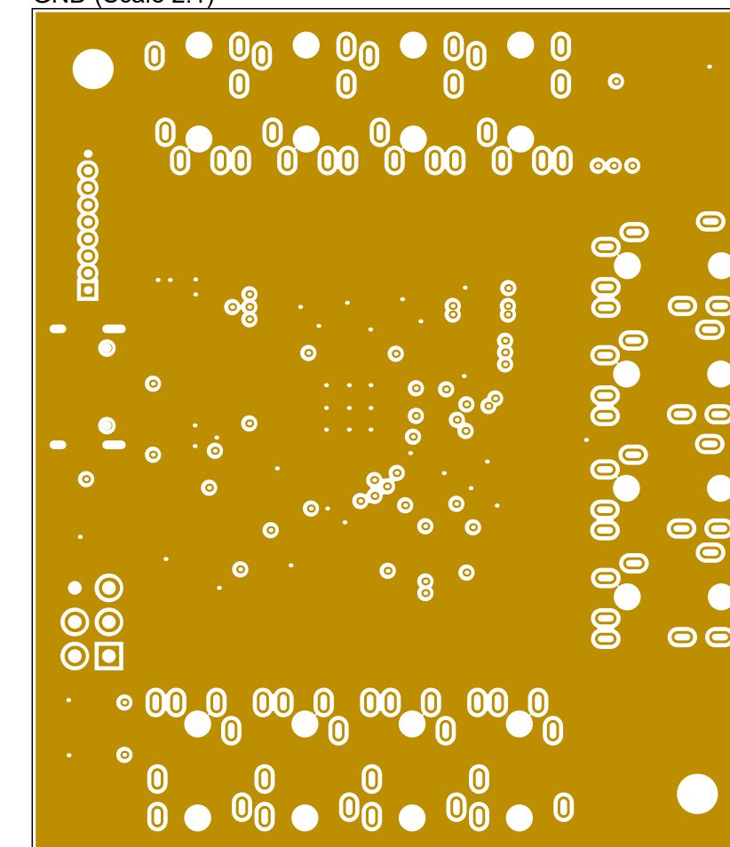
GND (Scale 2:1)
