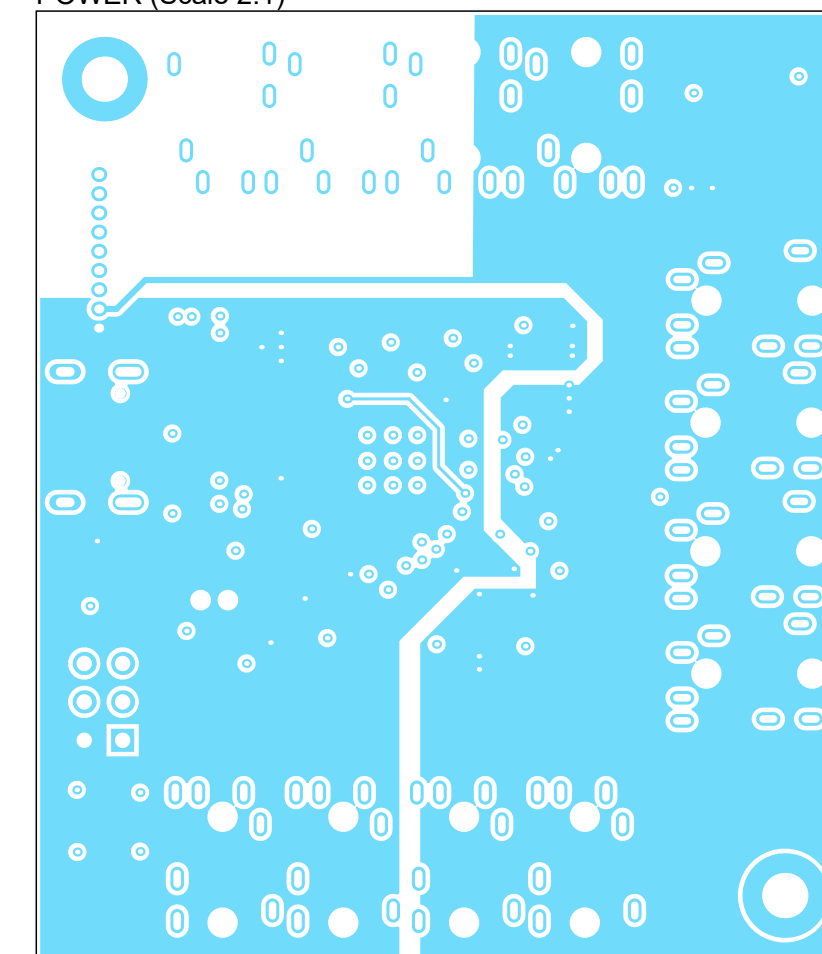
POWER (Scale 2:1)
