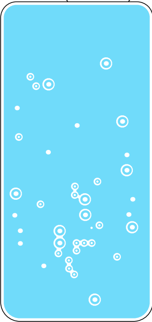
L3 - GND (Scale 4:1)
