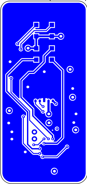
L4 - SIGNAL (Scale 4:1)
