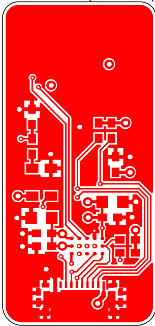
L1 - SIGNAL (Scale 4:1)
